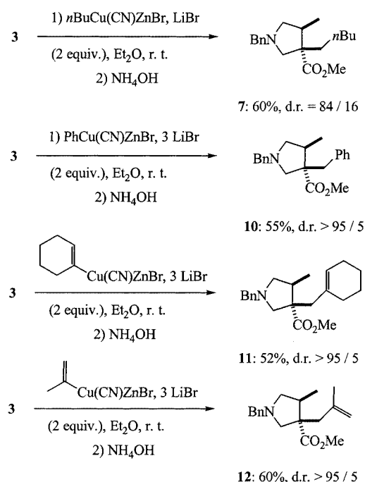
Scheme 8
