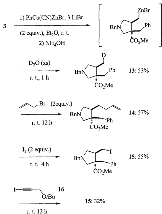
Scheme 9
