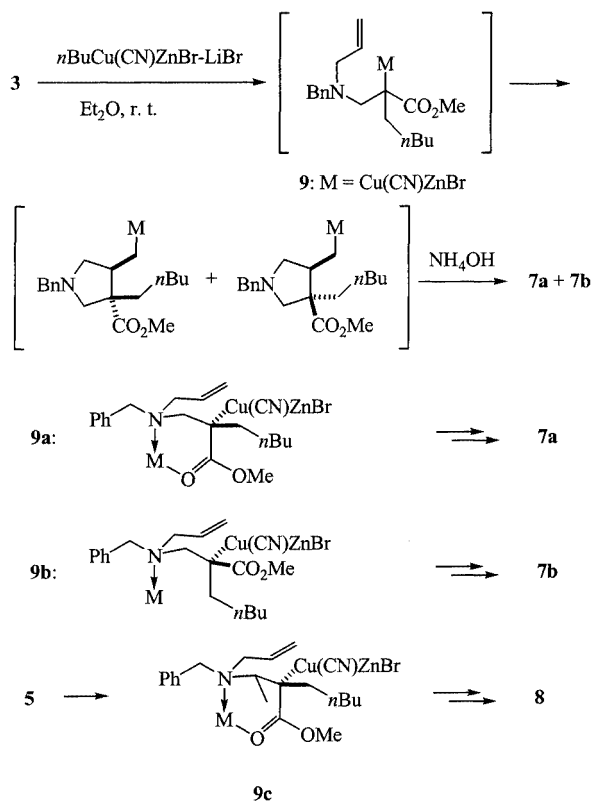
Scheme 7
